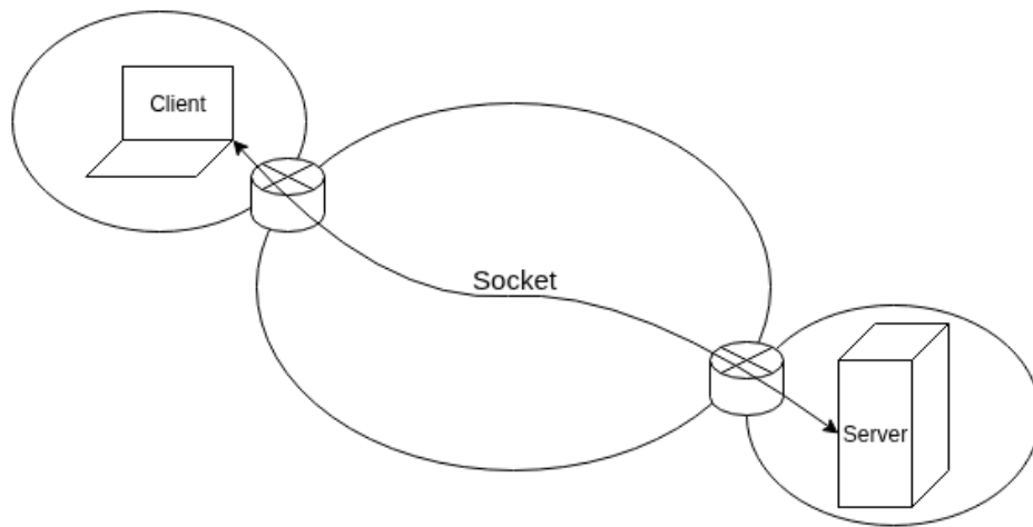
Figura 4.3: Modello client-server
